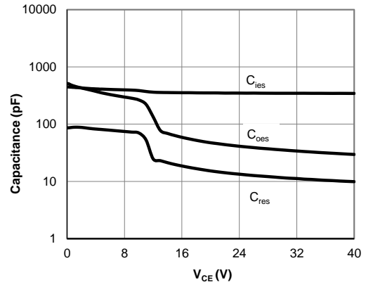
Figure 8: Capacitance Characteristic
