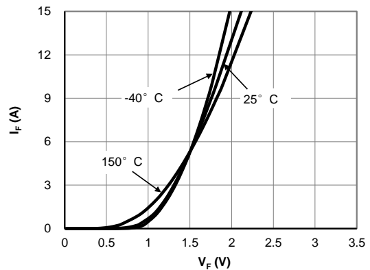
Figure 4: Diode Characteristic
