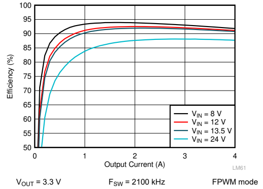
Figure 10-6. LM62440-Q1 Efficiency
