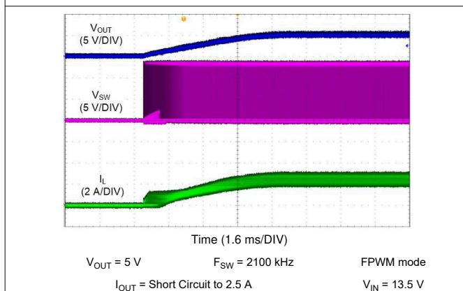
Figure 10-21. LM62440-Q1 Short Circuit Recovery
