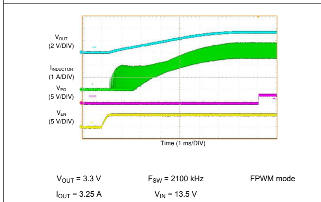
Figure 10-19. LM62440-Q1 Start-up with 3.25-A
