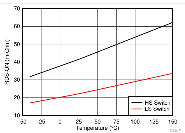
Figure 8-6. High-Side and Low-Side Switches R_{DS\_ON}
