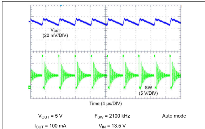
Figure 10-17. LM62440-Q1 Switching Waveform and V_{OUT} Ripple
