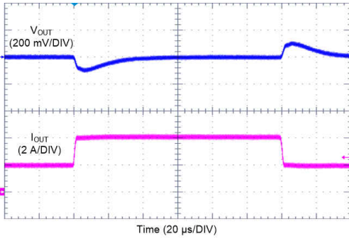
Figure 10-25. LM62440-Q1 Load Transient
