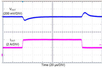
Figure 10-23. LM62440-Q1 Load Transient
