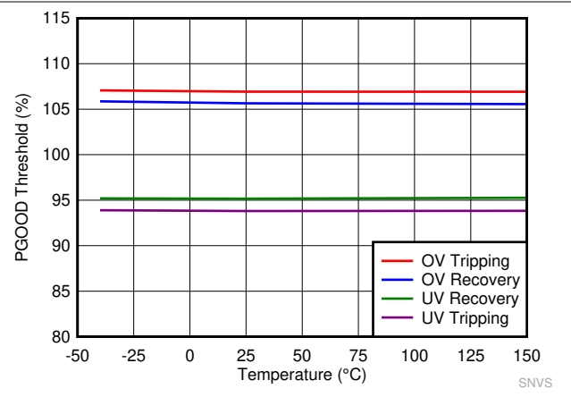
Figure 8-8. PGOOD Thresholds
