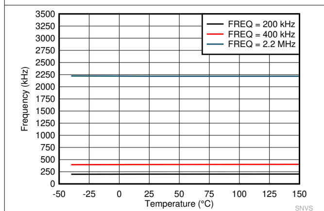
Figure 8-5. Switching Frequency Set by SYNC
