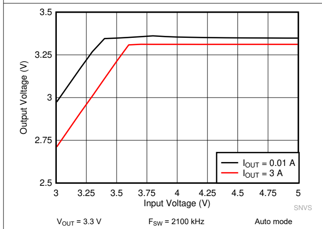
Figure 10-13. LM62440-Q1 Dropout Curve
