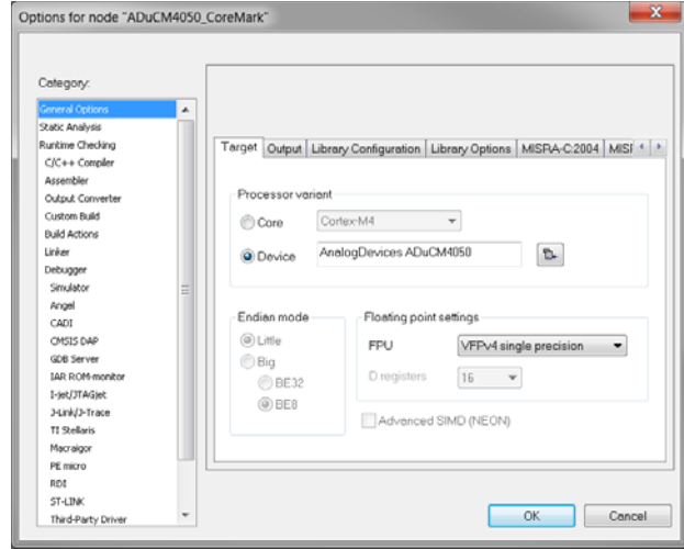
Figure 3. General Options—Target Configuration
