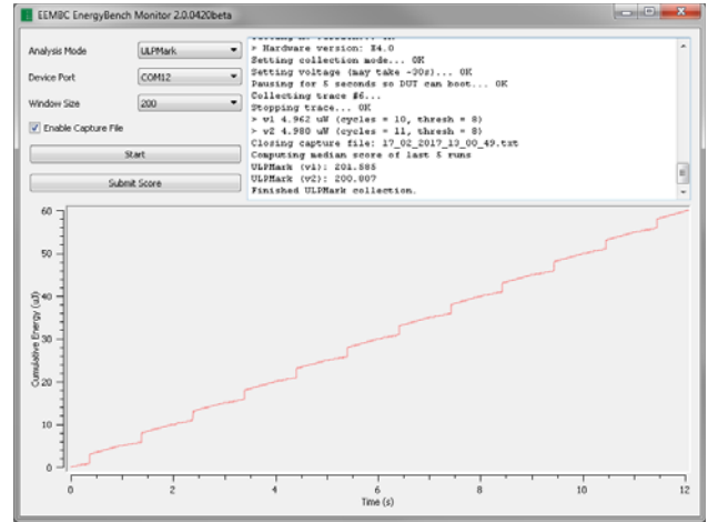
Figure 31. ULPMark-CP Score
