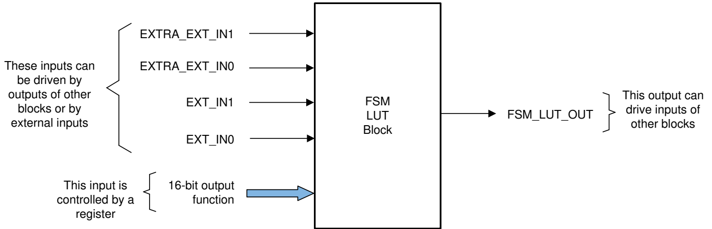
Figure 29-12. FSM LUT Block
