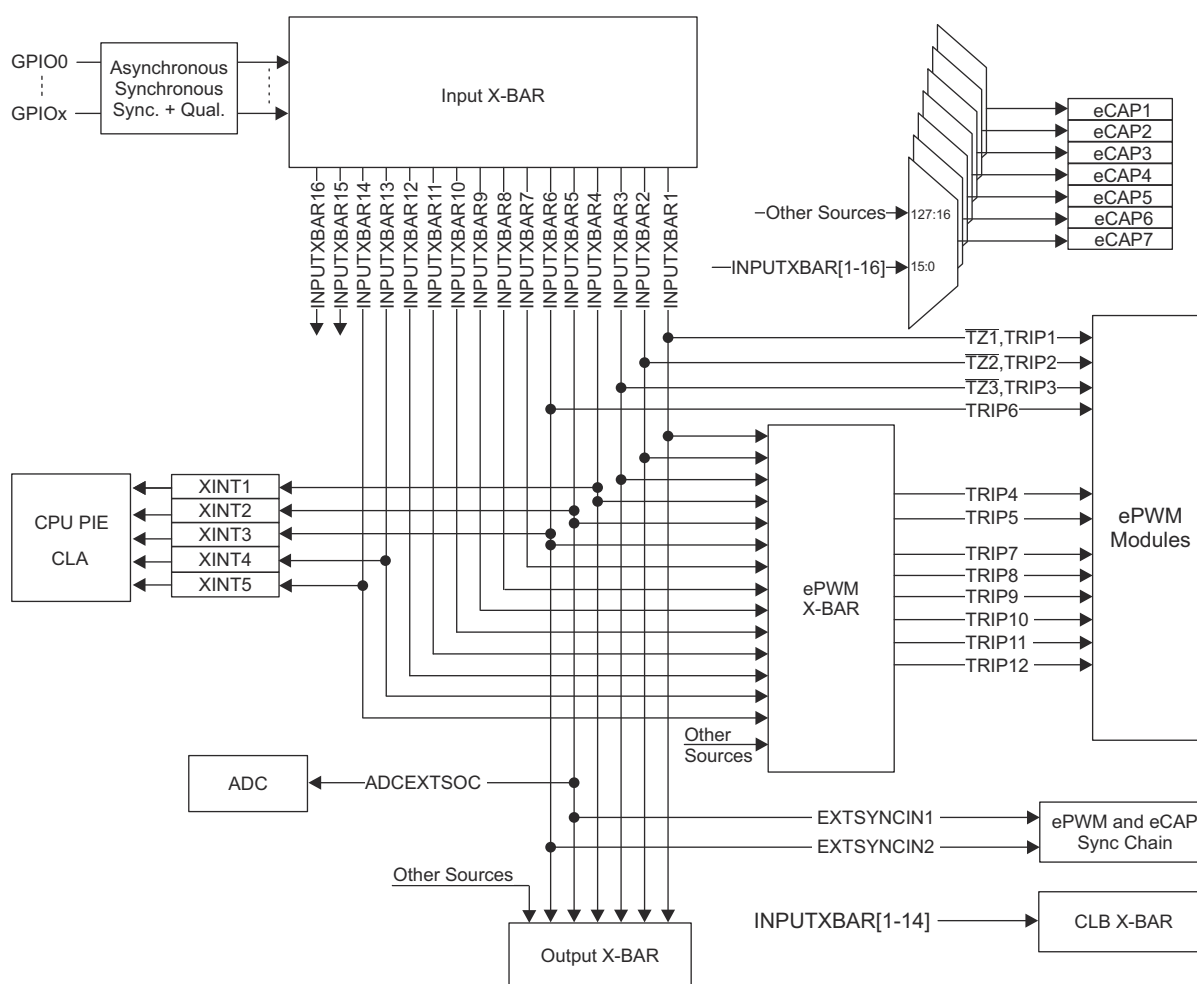
Figure 9-1. Input X-BAR
