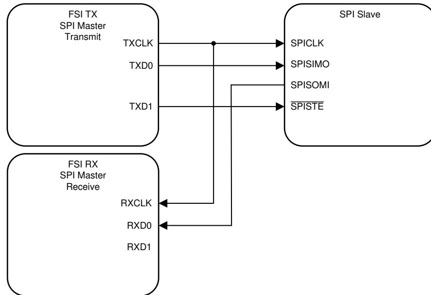
Figure 28-12. FSITX and FSIRX as SPI Master, Full Duplex
