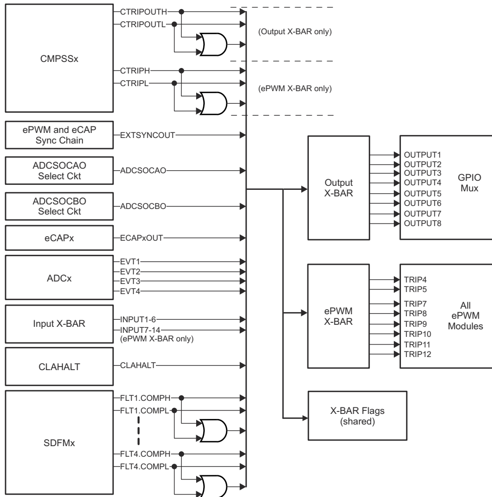
Figure 18-58. ePWM X-BAR
