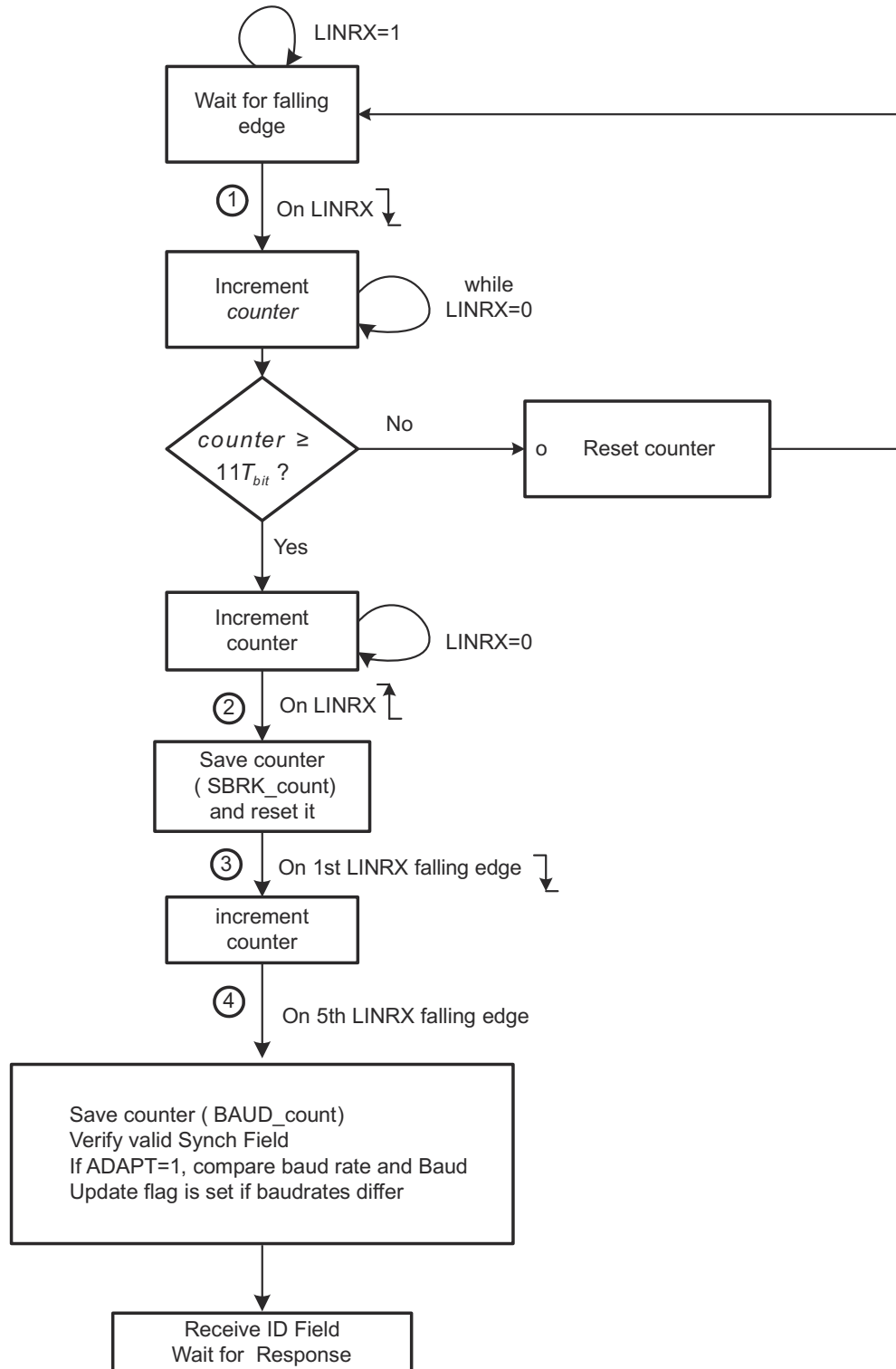
Figure 27-18. Synchronization Validation Process and Baud Rate Adjustment
