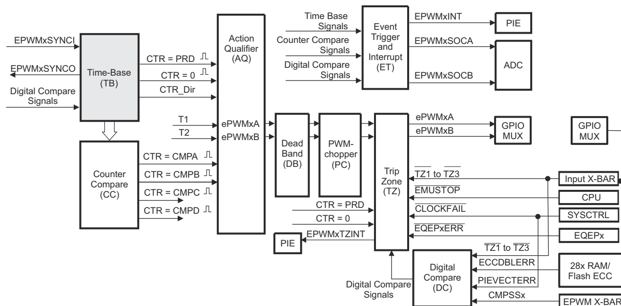
Figure 18-4. Time-Base Submodule
