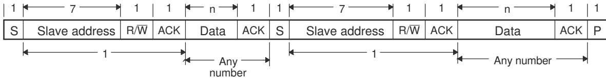
Figure 24-13. Repeated START Condition (in This Case, 7-Bit Addressing Format)
