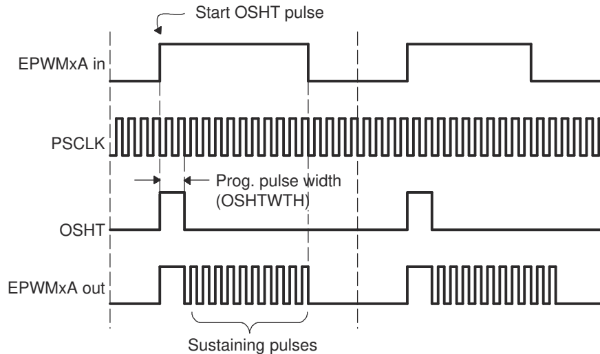
Figure 18-39. PWM Chopper Submodule Waveforms Showing the First Pulse and Subsequent Sustaining Pulses
