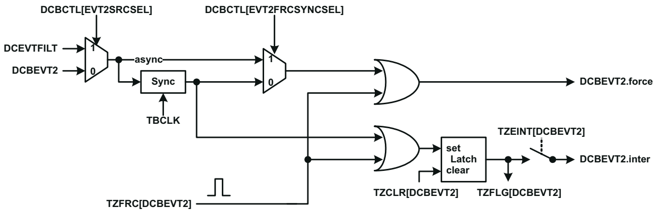
Figure 18-54. DCBEVT2 Event Triggering
