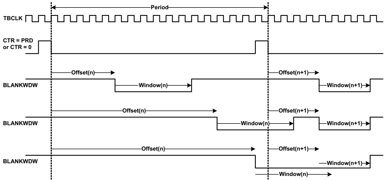
Figure 18-56. Blanking Window Timing Diagram
