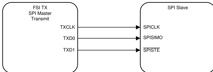
Figure 28-10. FSITX as SPI Master, Transmit Only
