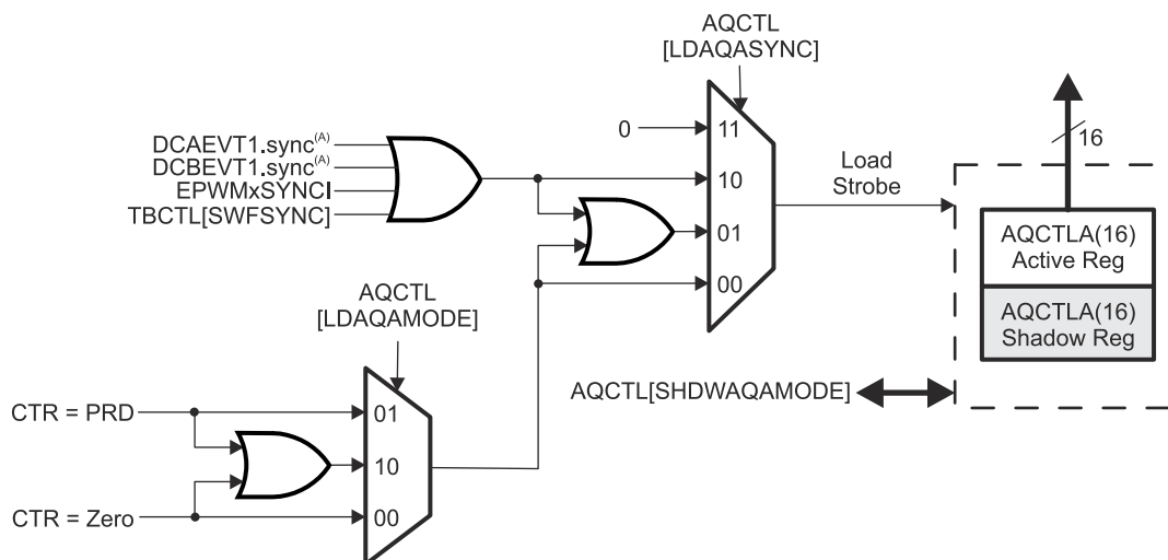
Figure 18-23. AQCTL[SHDWAQAMODE]
