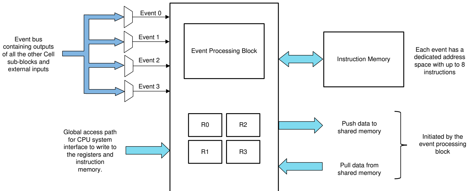
Figure 29-17. High Level Controller Block
