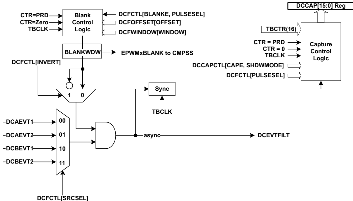
Figure 18-55. Event Filtering
