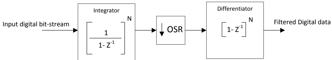
Figure 17-5. Simplified Sinc Filter Architecture
