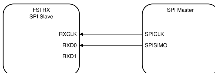
Figure 28-11. FSIRX as SPI Slave, Receive Only
