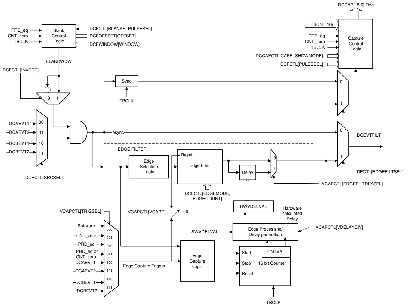
Figure 18-57. Valley Switching
