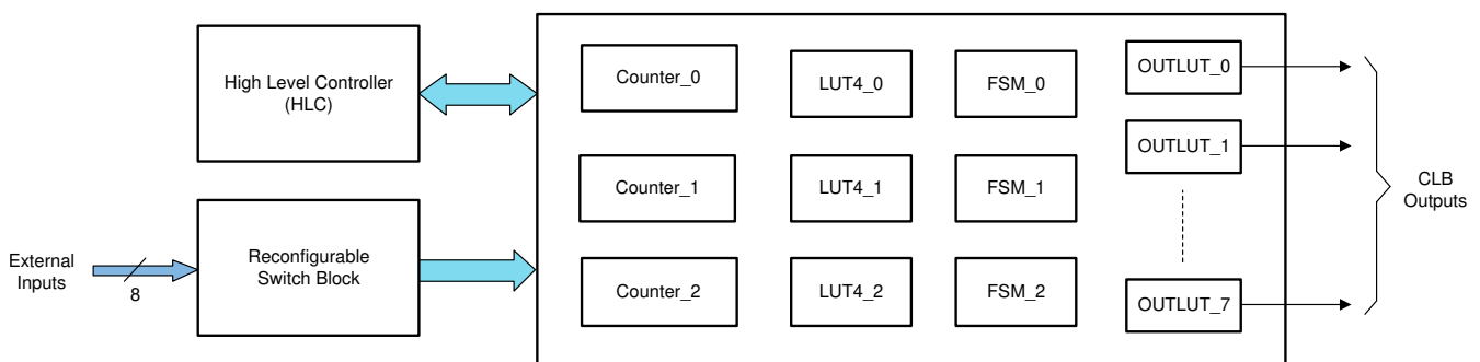
Figure 29-8. CLB Tile Submodules
