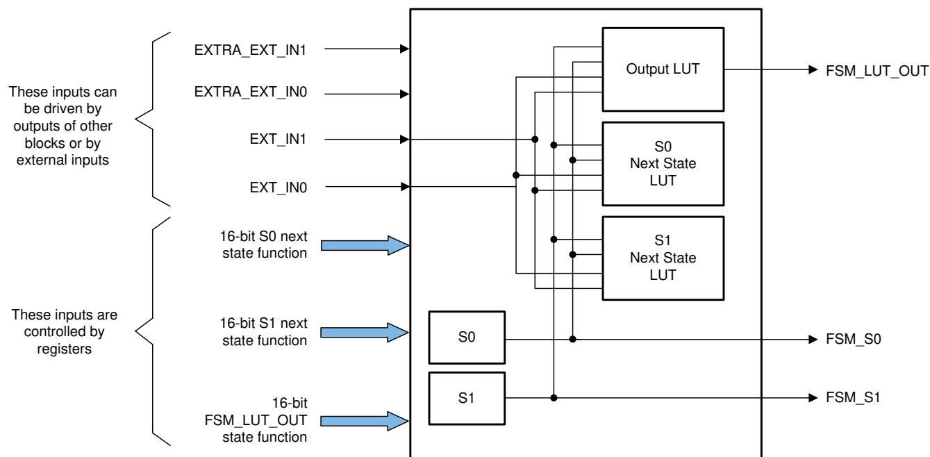
Figure 29-11. FSM Block
