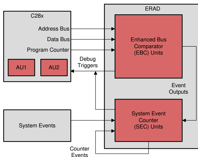
Figure 11-1. ERAD Overview
