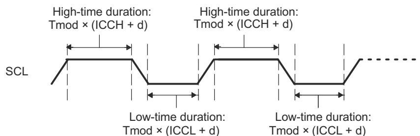
Figure 24-4. Roles of the Clock Divide-Down Values (ICCL and ICCH)
