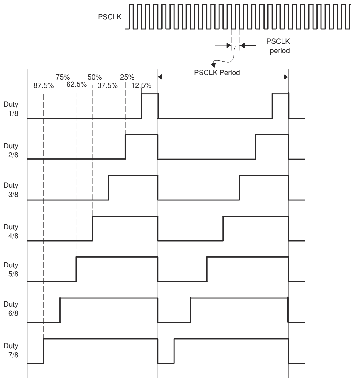
Figure 18-40. PWM Chopper Submodule Waveforms Showing the Pulse Width (Duty Cycle) Control of Sustaining Pulses
