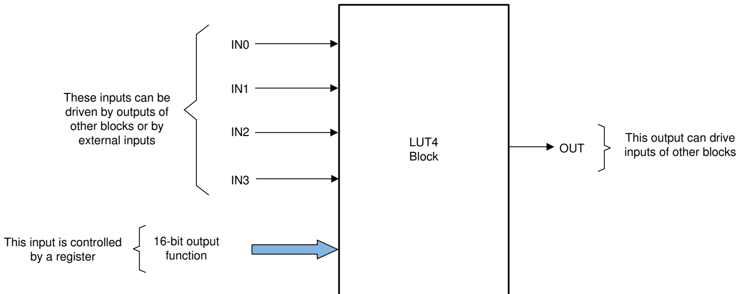
Figure 29-13. LUT4 Block
