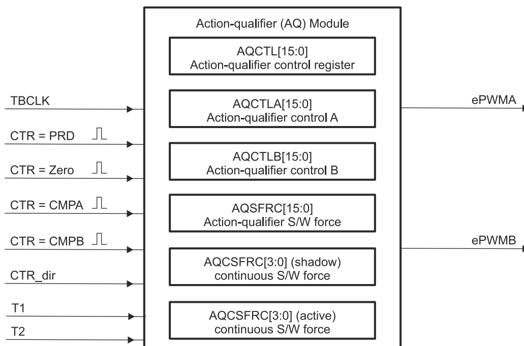
Figure 18-21. Action-Qualifier Submodule Inputs and Outputs
