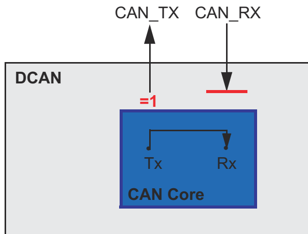
Figure 26-6. CAN Core in Loopback Combined with Silent Mode
