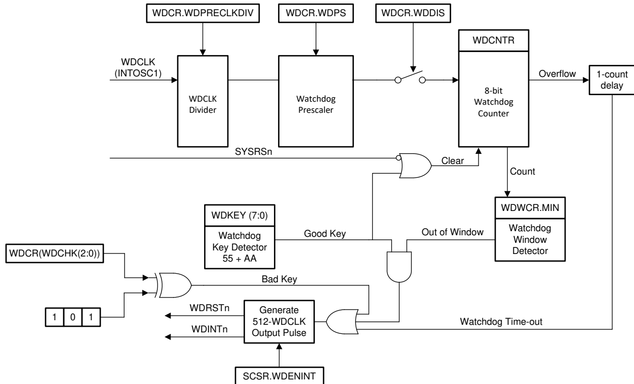
Figure 3-11. Watchdog Timer Module
