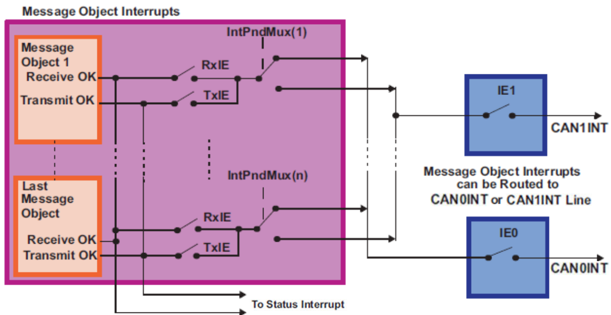
Figure 26-8. CAN Interrupt Topology 2
