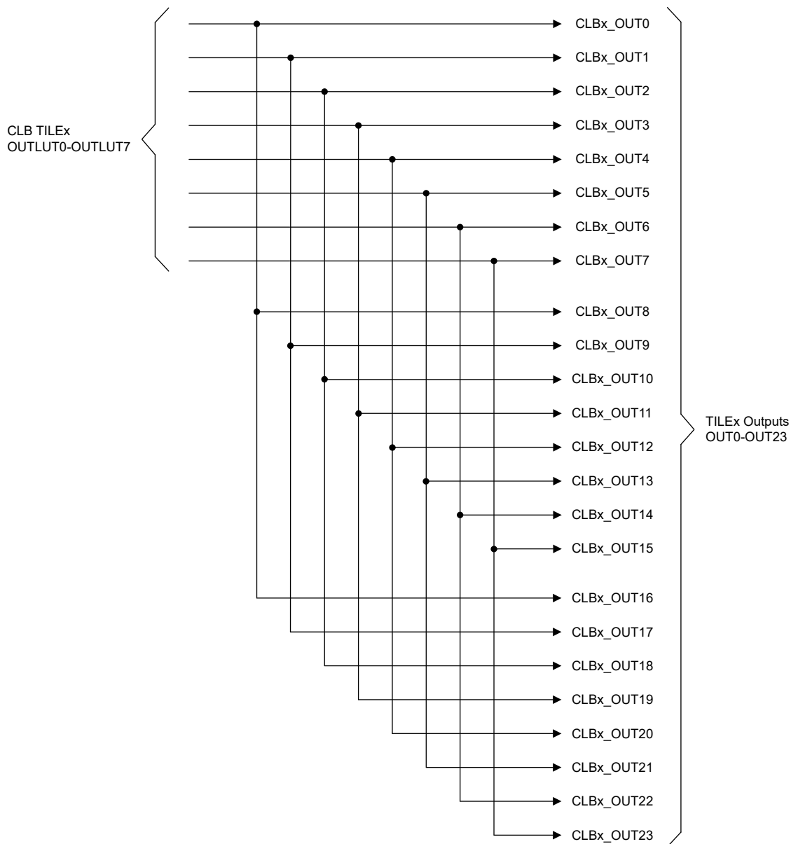
Figure 29-6. CLB Outputs
