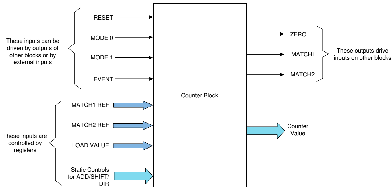
Figure 29-9. Counter Block
