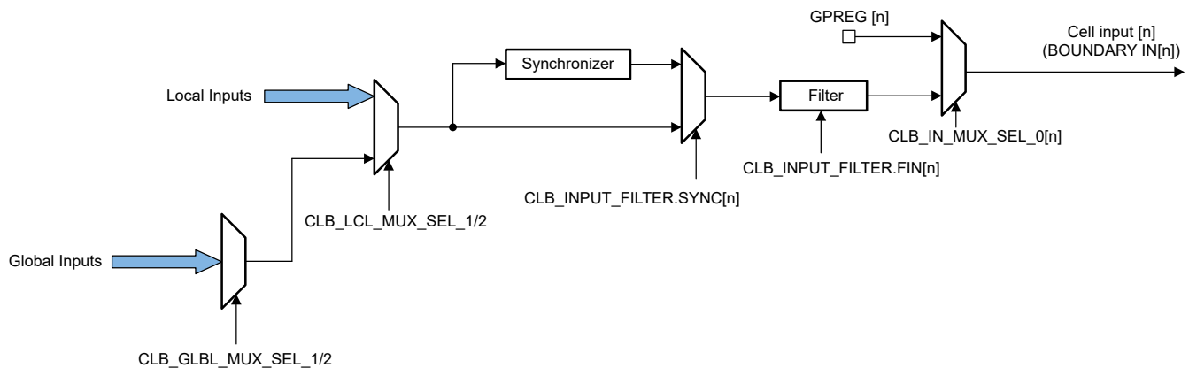
Figure 29-4. CLB Input Mux and Filter
