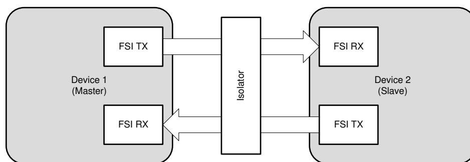
Figure 28-13. Point to Point Connection
