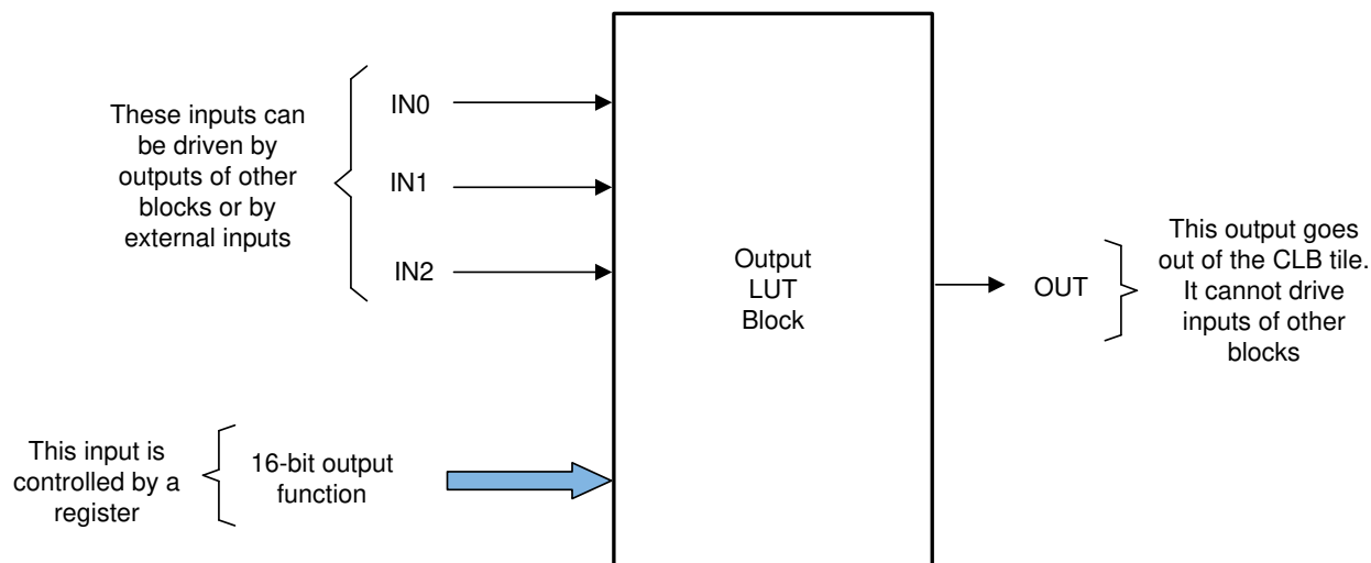
Figure 29-14. Output LUT Block
