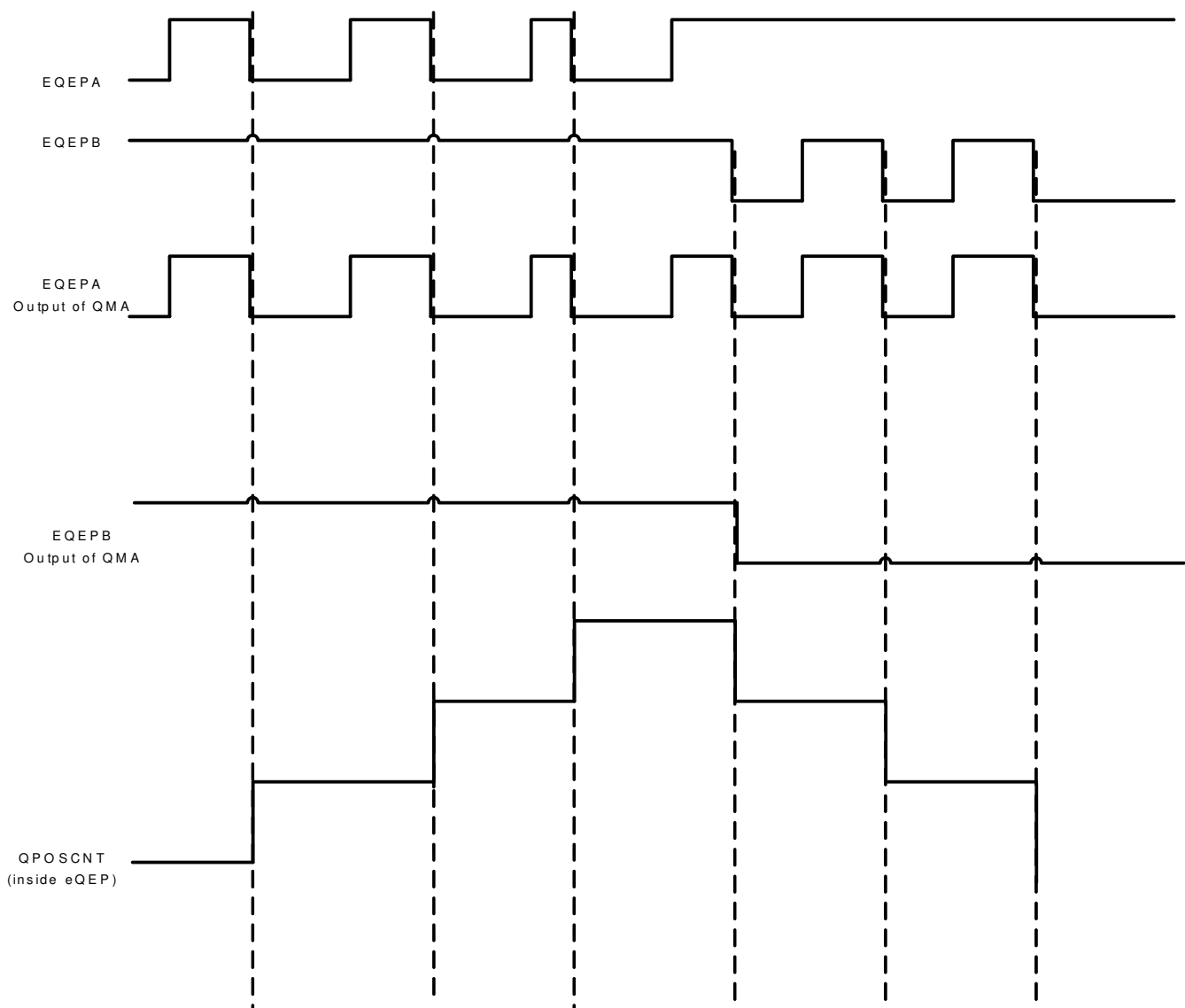
Figure 21-21. QMA Mode-1
