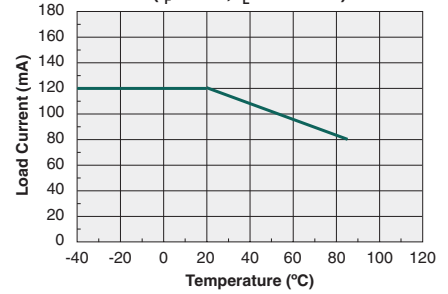
Maximum Load Current vs. Temperature ( I_F=0\text{mA} , I_L=AC\text{ Peak} )
