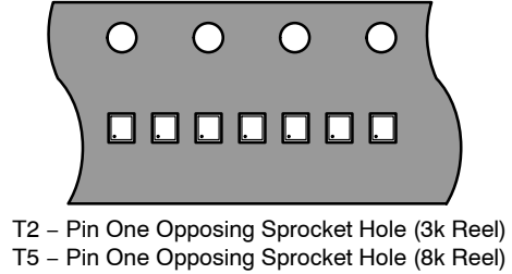
Figure 40. XLLGA, DFN
