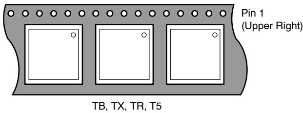
Figure 45. SIP
