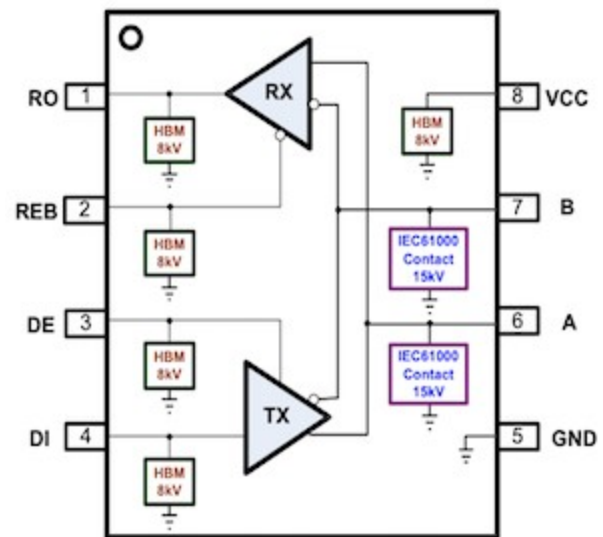
Functional Block of AZRS3080E
