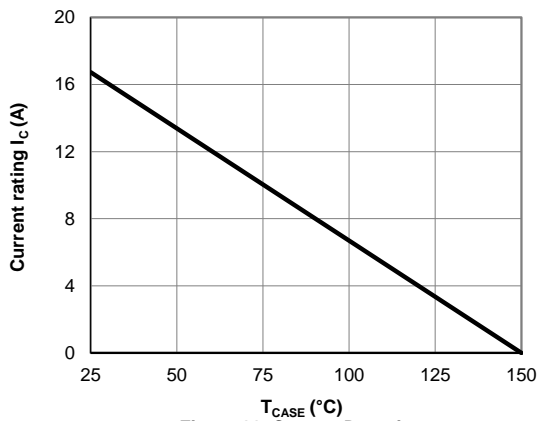
Figure 11: Current De-rating
