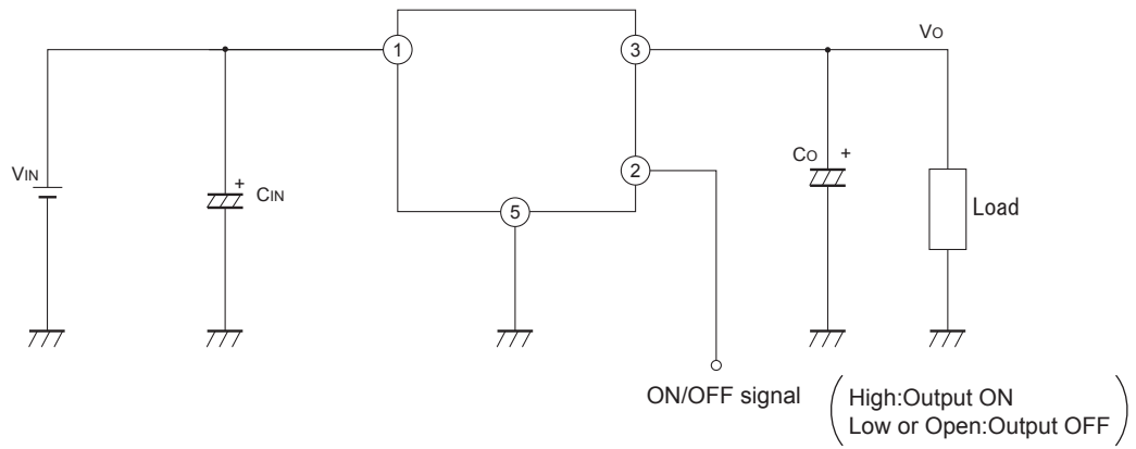
Fig.1 Typical Application
