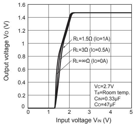
Fig.15 Output Voltage vs. Input Voltage (PQ015EN01ZPH)
