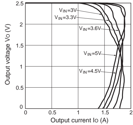
Fig.7 Overcurrent Protection Characteristics (PQ025EN01ZPH)
