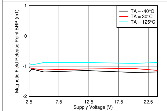
Figure 7-3. BRP_Z Threshold vs. V CC
