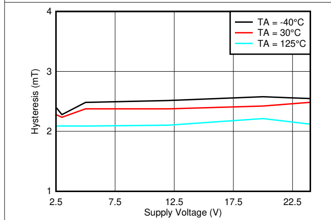
Figure 7-5. Hysteresis_Z vs. V CC
