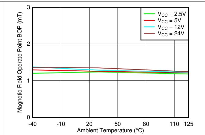
Figure 7-2. BOP_Z Threshold vs. Temperature
