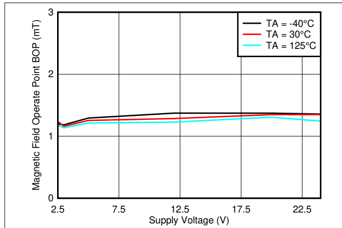
Figure 7-1. BOP_Z Threshold vs. V CC
