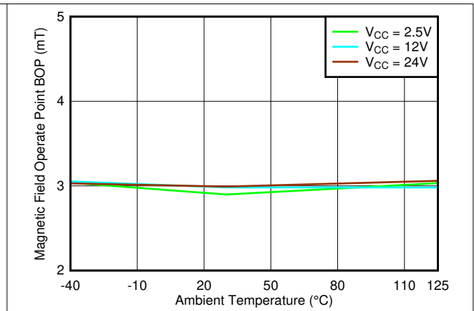
Figure 7-40. B_{OP\_Z} Threshold vs. Temperature
