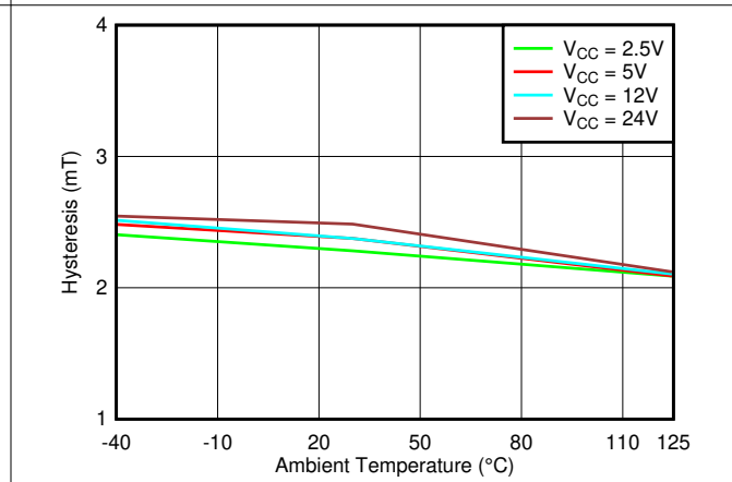
Figure 7-6. Hysteresis_Z vs. Temperature
