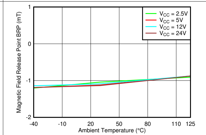
Figure 7-4. BRP_Z Threshold vs. Temperature
