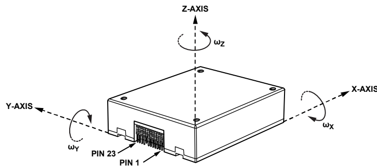
Figure 34. Gyroscope Axis and Polarity Assignments
