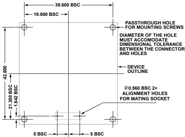
Figure 46. Suggested PCB Layout Pattern, Connector Down
