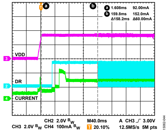
Figure 48. Transient Current Demand, Startup (DR Means Data Ready)
