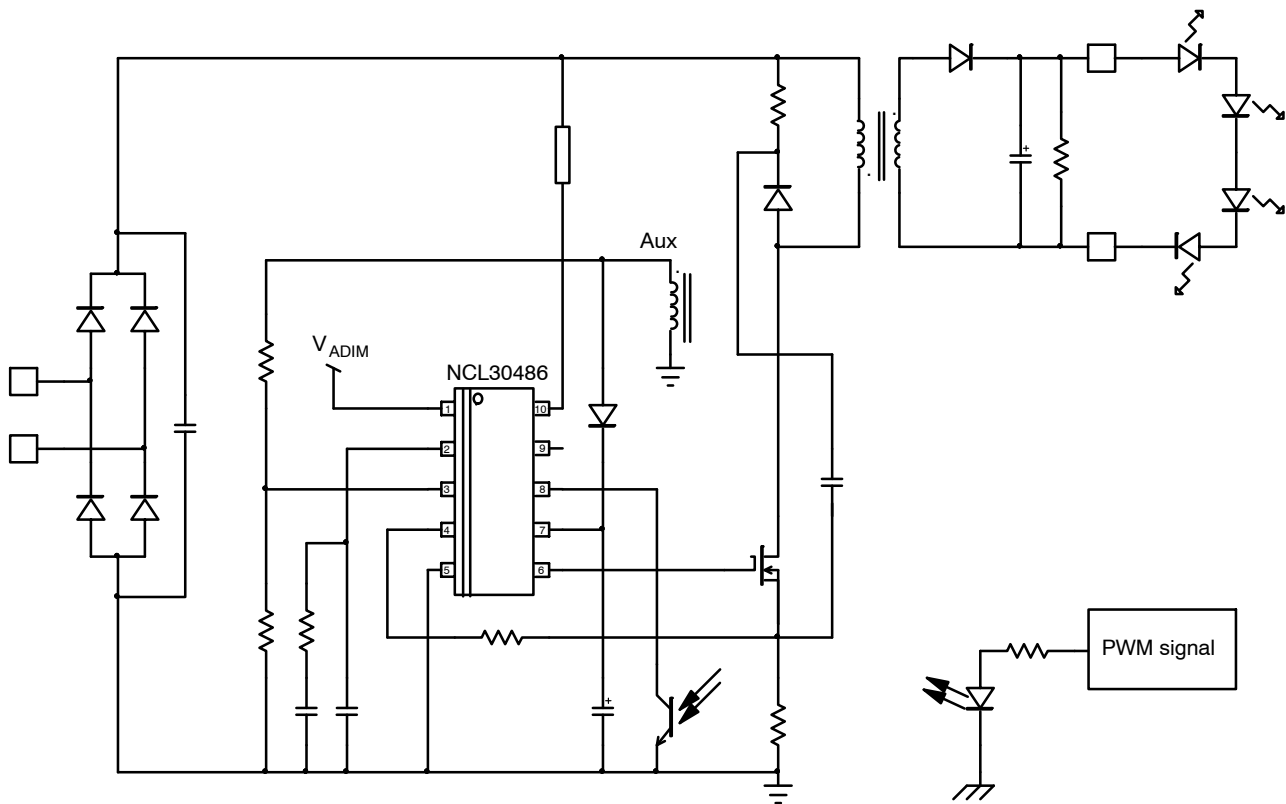
Figure 1. Typical Application Schematic for NCL30486
